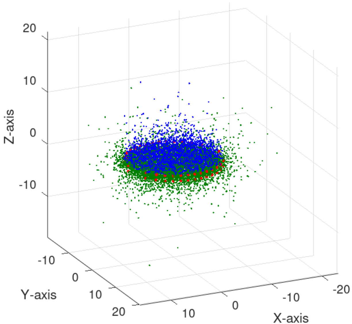
Figure 6: Problem2-h1.png: cylinder e^- radiation in green and blue points, where only the blue points refer to the detected points. The visual count of blue points is noticeably large compared to the green emitted dots beyond the cylinder. This for a cylinder of height 1 [mm].
